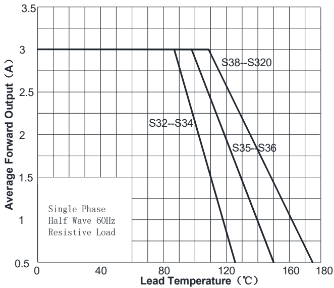
FIG1:Io-TL Curve
